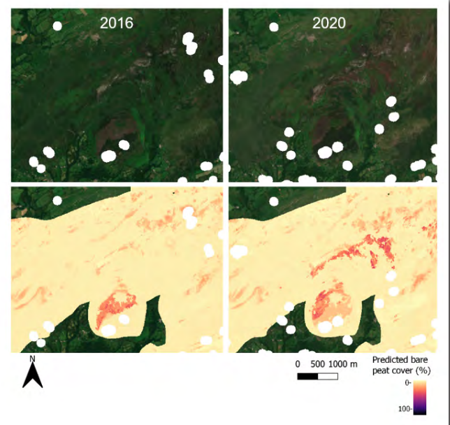
Figure 1: Time-series maps displaying changes in the predicted amount of bare peat cover (bottom row) between 2016 and 2020 for a site in the Brecon Beacons, Wales (top row), plotted against Sentinel-2 imagery. White areas represent areas of cloud.
