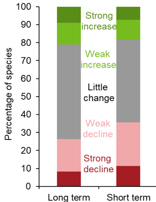
Figure 2: The proportion of priority species in each trend category based on mean change in occupancy over both a) the long term (all years) and b) the short term (the most recent 5 years)
