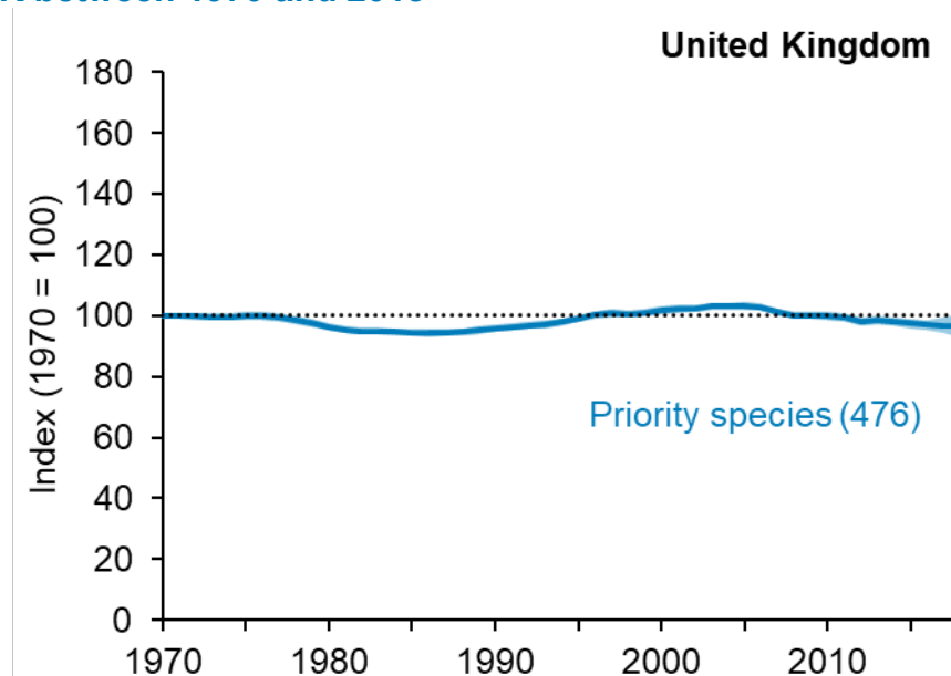
Figure 1: Change in the occupancy (proportion of occupied sites) of priority species in the UK between 1970 and 2018
