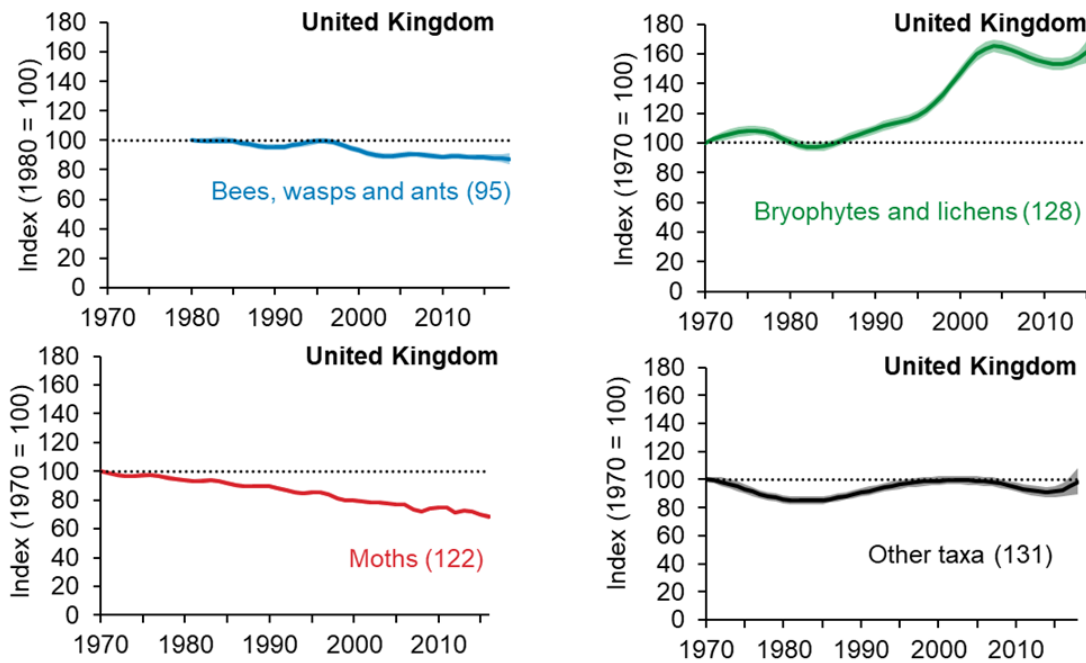
Figure 3: Change in distribution of UK priority species, by taxonomic group, 1970 3 to 2018
