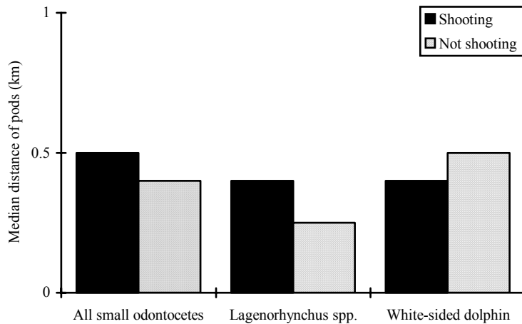
Figure 11 Median distance of marine mammals from the airguns in relation to seismic activity during site surveys
