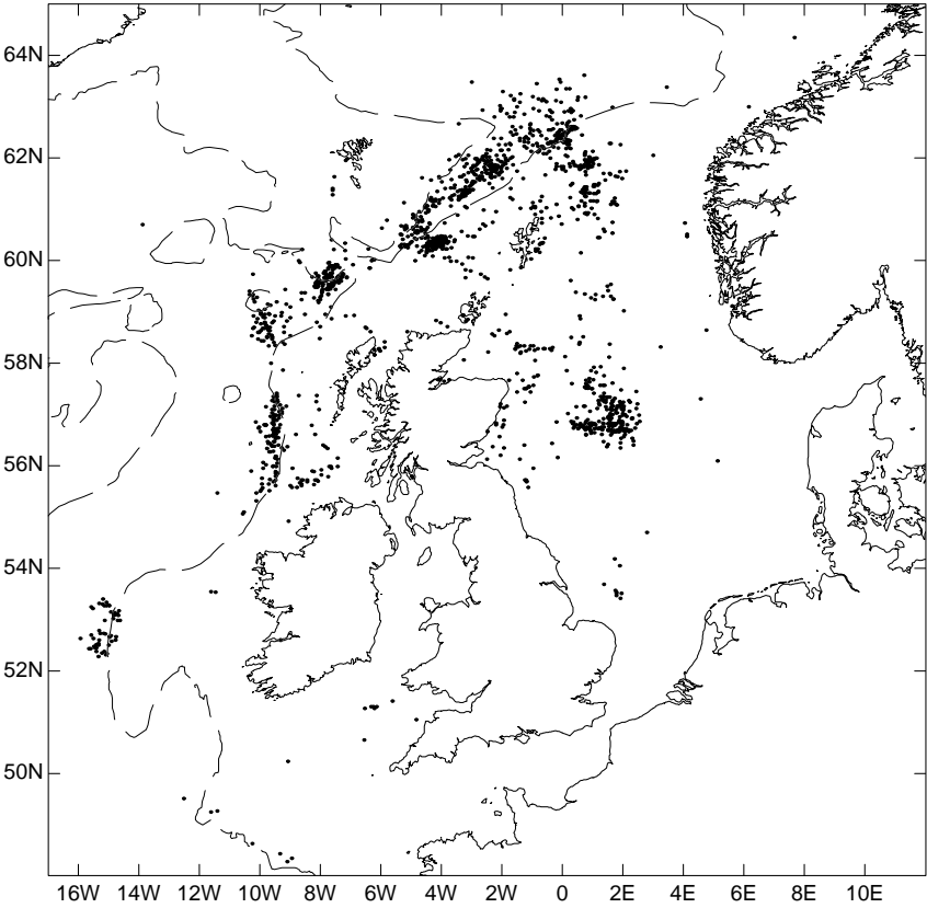
Figure 16 Marine mammal sightings from seismic survey vessels, 1998-2000.
