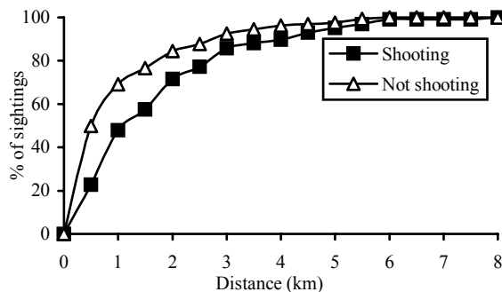
Figure 12 Proportion of marine mammal sightings occurring within specified distances of the airguns, in relation to seismic activity (excluding site surveys).
