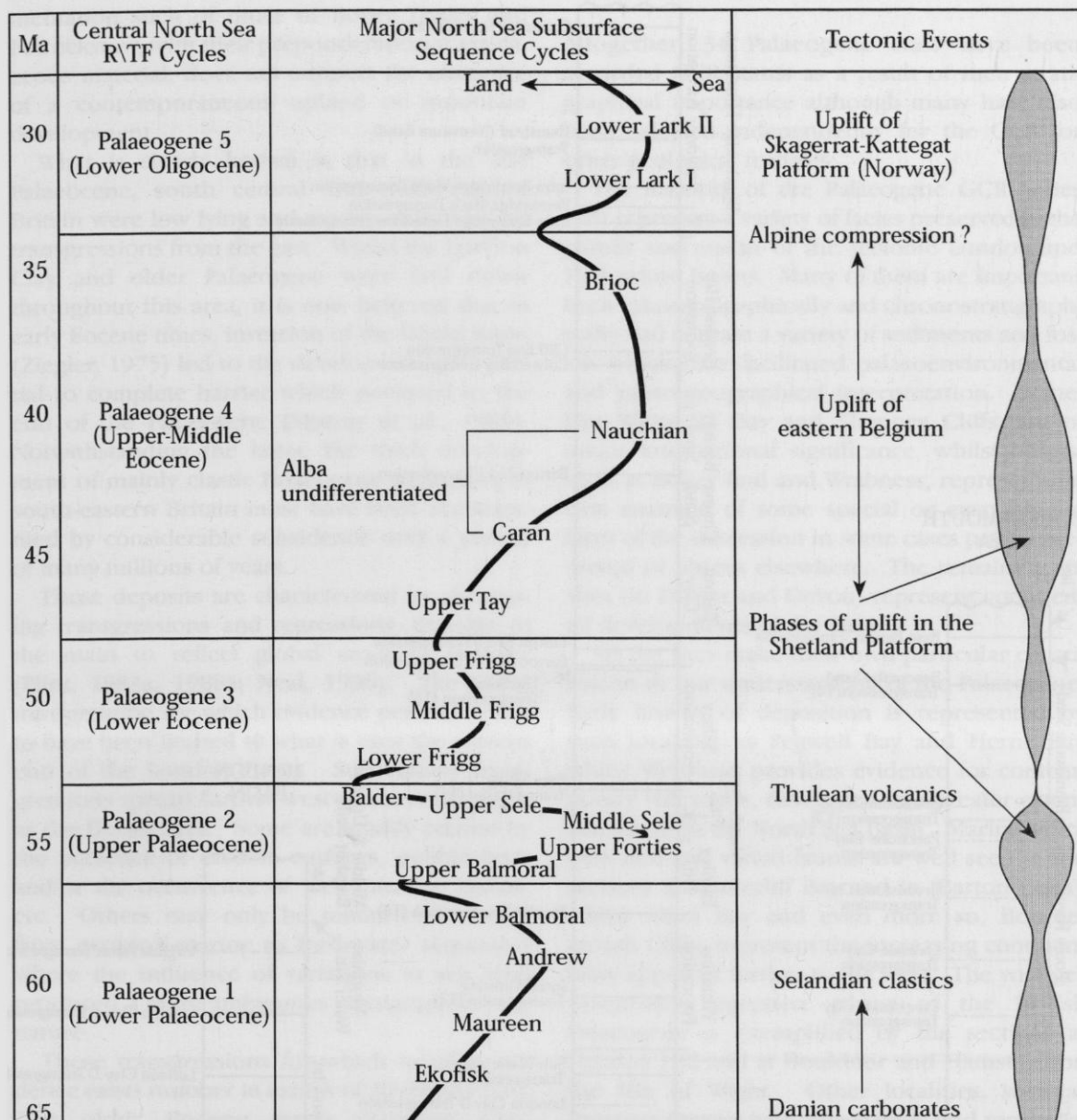
Figure 2.5 Relative sea level curve to show major regressive/transgressive (R/TF) cycles and depositional sequences for the central North Sea, and its relationship to major tectonic events (after Neal, 1996).
