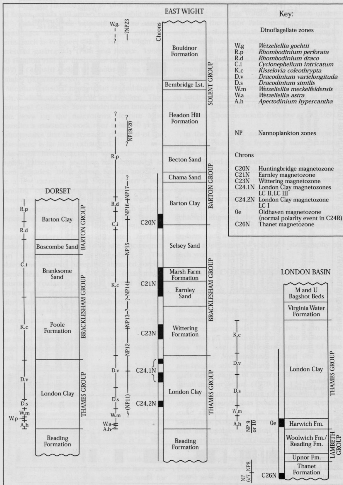
Figure 2.3 Comparative succession of the Palaeogene strata in the Hampshire and London Basins, to show the relationship between the major lithostratigraphical units and magnetozone, nannoplankton zones and dinoflagellate zones (after various authors).
