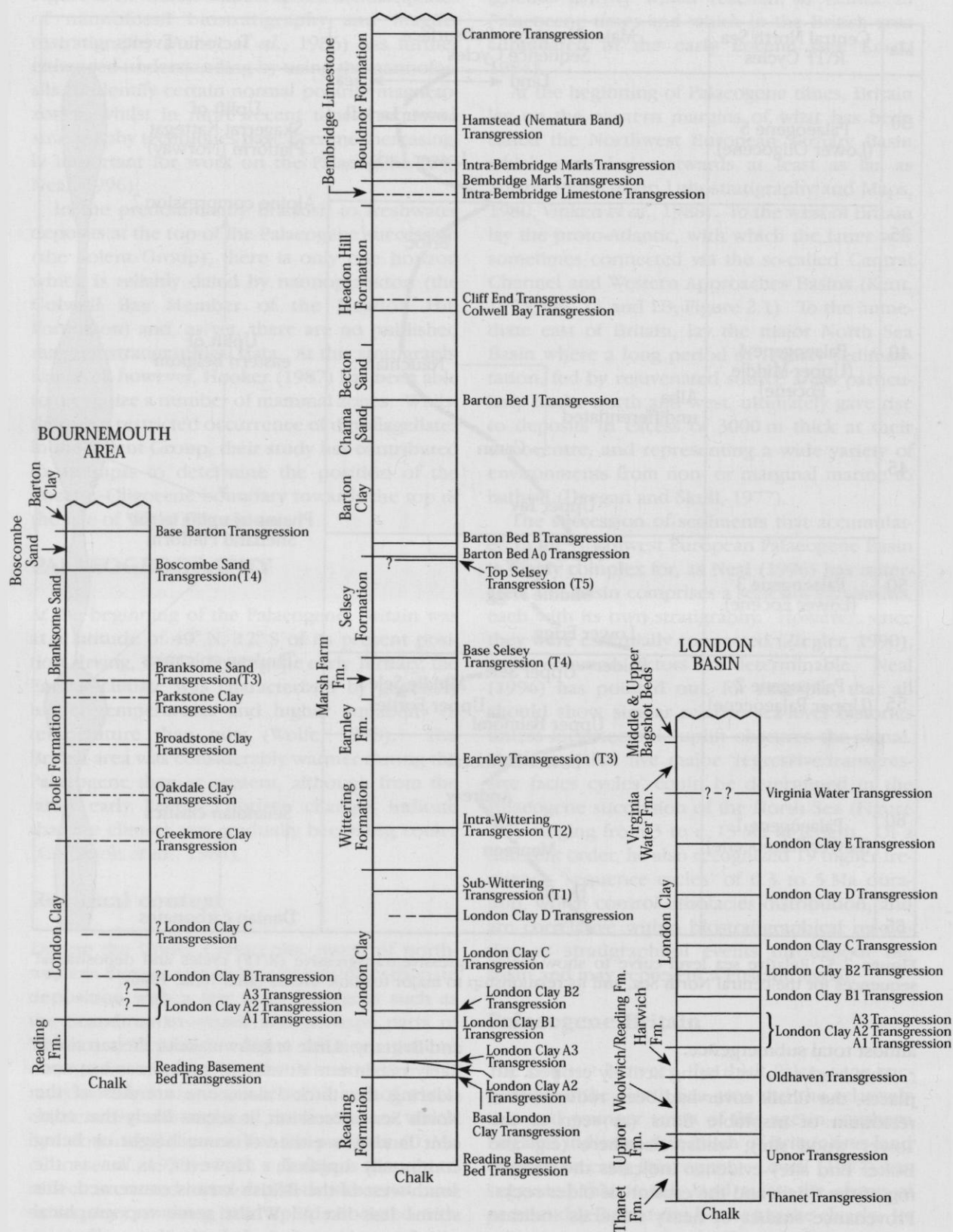
Figure 2.6 Simplified representation of the relationship between transgressive events and the major Palaeogene lithostratigraphical units in southern England, based on a variety of sources. (T1) to (T5) numbering after Plint (1983a). Dot-dashed lines represent relatively minor events.
