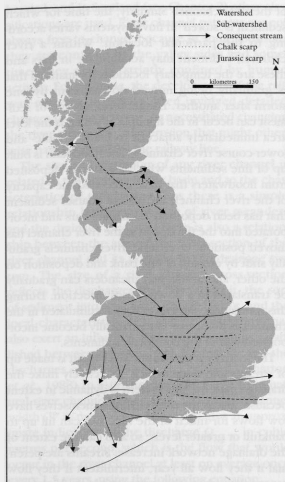
Figure 1.2 The original drainage pattern for England and Wales as initiated by Early Tertiary uplift of the late Cretaceous sea floor (Brown, 1960), and the initial watersheds and initial drainage of Scotland (after Sissons, 1967).
