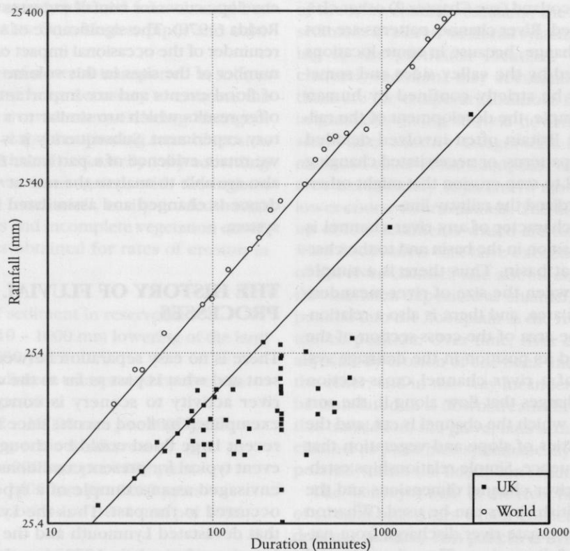
Figure 1.3 Rainfall magnitude-duration relationships for the world and the UK. The largest falls (from Rodda, 1970) and magnitude-duration relationships of geomorphologically significant UK floods, where known, are given.
