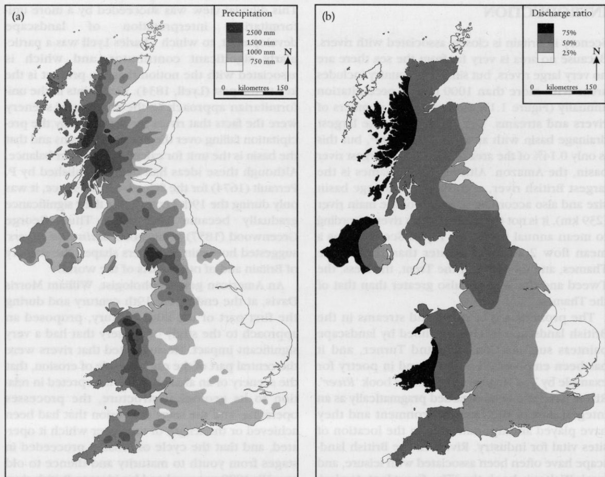
Figure 1.1 (a) Annual precipitation for the whole of Britain (after Ward, 1981). (b) The discharge ratio for the whole of Britain (after Ward, 1981).
