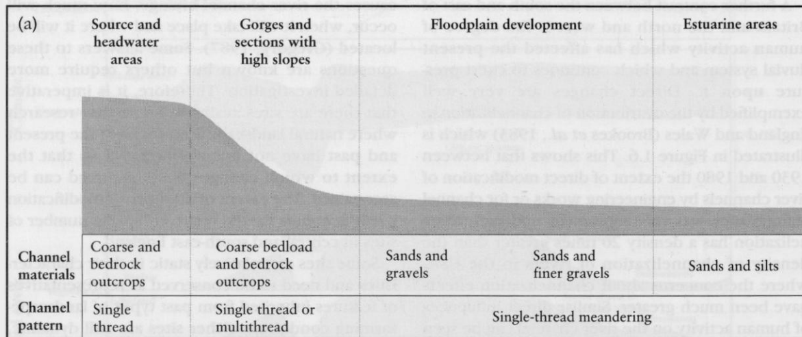
Figure 1.5 (a) An idealized section showing the relationship between river profile, channel materials and channel pattern. (After Smith and Lyle, 1979.)
