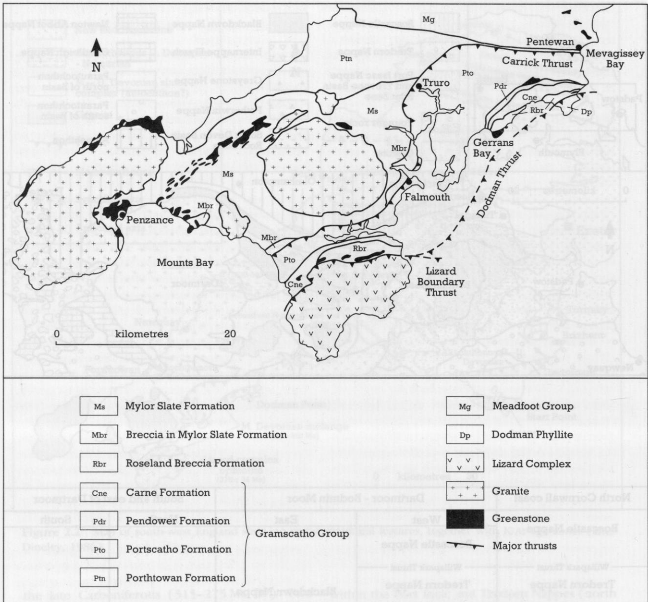
Figure 2.4 Geological map of south Cornwall showing various allochthonous units, including the Lizard Complex, resting on the northern parautochthon of the Porthtowan Formation and Mylor Slate Formation (after Holder and Leveridge, 1986).
