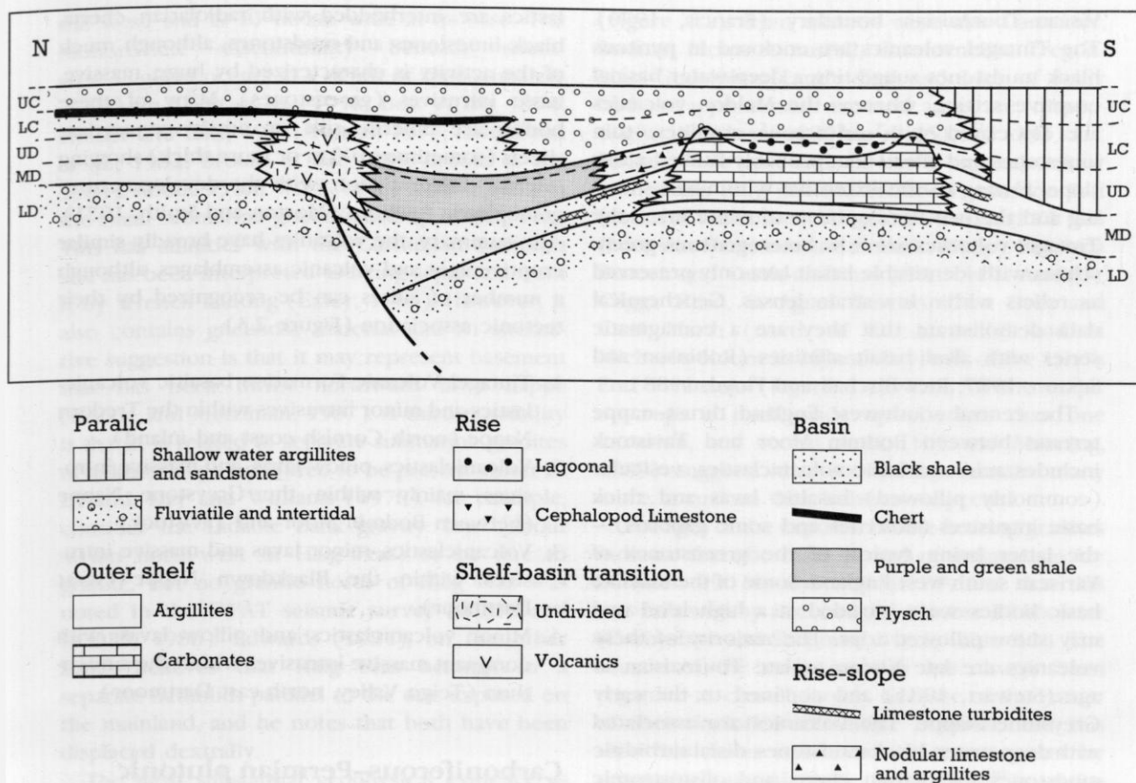
Figure 2.7 Generalized facies relationships throughout the Devonian and Carboniferous of central south-west England (after Selwood and Thomas, 1986b). LD = Lower Devonian; MD = Middle Devonian; UD = Upper Devonian; LC = Lower Carboniferous; UC = Upper Carboniferous.
