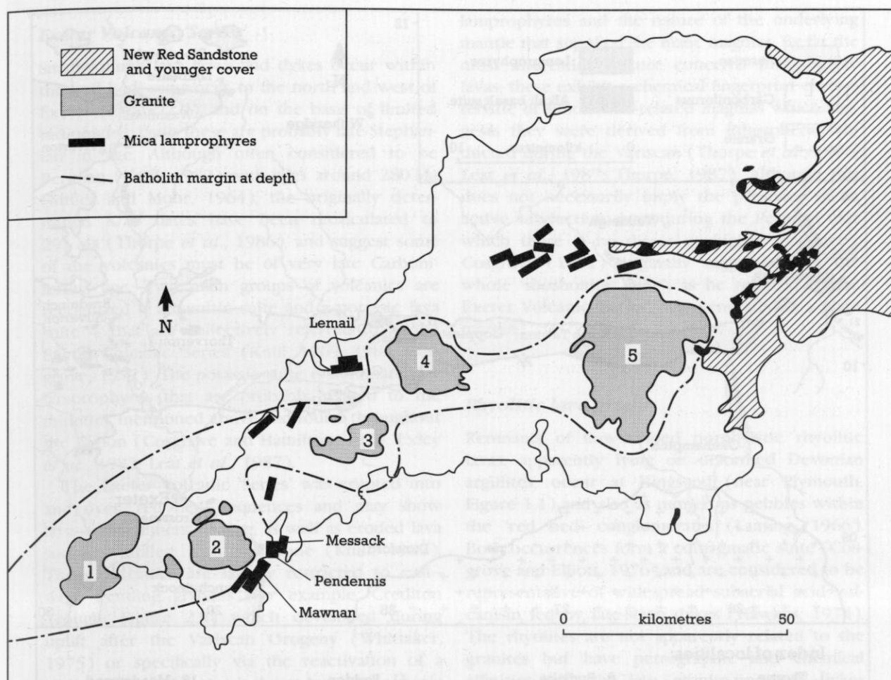
Figure 2.8 Geological outline map of south-west England, showing the distribution of mica lamprophyres relative to the exposed Cornubian granite batholith (grey) and its geophysically determined margin (after Leat et al. , 1987). The Exeter Volcanic 'Series' is shown within the New Red Sandstone outcrop and younger Mesozoic rocks (diagonal ruling). 1 = Land's End Granite; 2 = Carnmenellis Granite; 3 = St Austell Granite; 4 = Bodmin Moor Granite; 5 = Dartmoor Granite.
