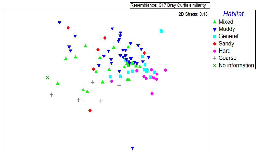
Figure 1. Preliminary nMDS ordination against habitat preferences. Each point represents a species although for clarity labels have been omitted. The symbols represent habitat preferences.
