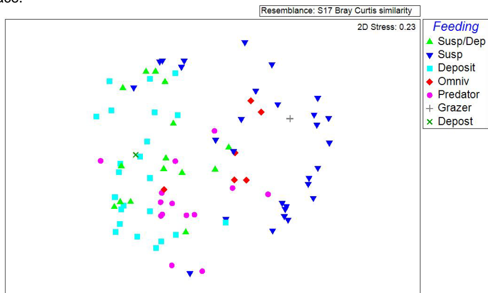
Figure 3. Non-MDS ordination against all biological traits. Each point represents a species although for clarity labels have been omitted. The symbols represent the dominant feeding type.
