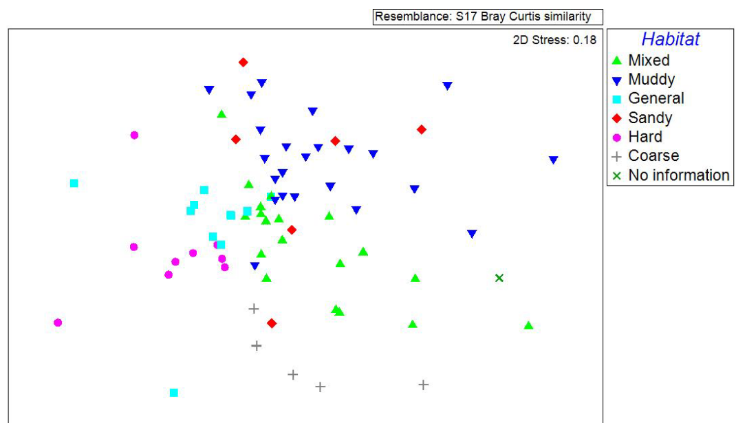
Figure 2. Non-MDS ordination against depth and substratum preferences. Each point represents a species although for clarity labels have been omitted. The symbols represent habitat preferences.
