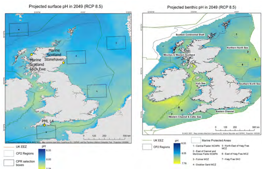
Projected surface pH and seabed pH around the UK in 2049
