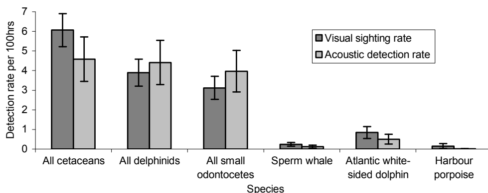
Figure 3.12. Mean detection rate (and standard error) per 100 hours monitoring for visual and acoustic monitoring.
