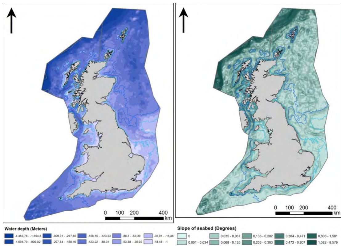
Figure 7. Bathymetry and slope of sea floor used as predictor variables
