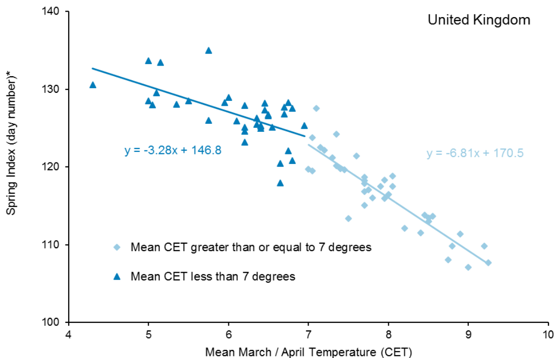
Figure B4ii. Relationship between Spring Index and Central England Temperature, 1891 to 1947, and 1999 to 2018
